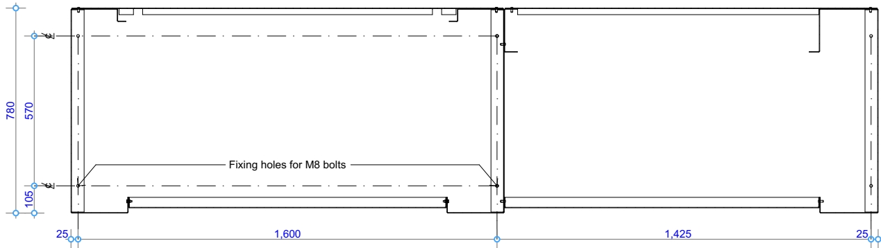
Fixing Set-out - Plan View
