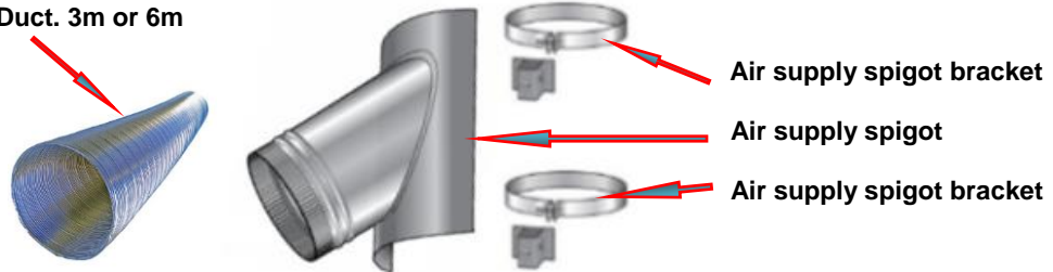
Air supply duct and bracket
