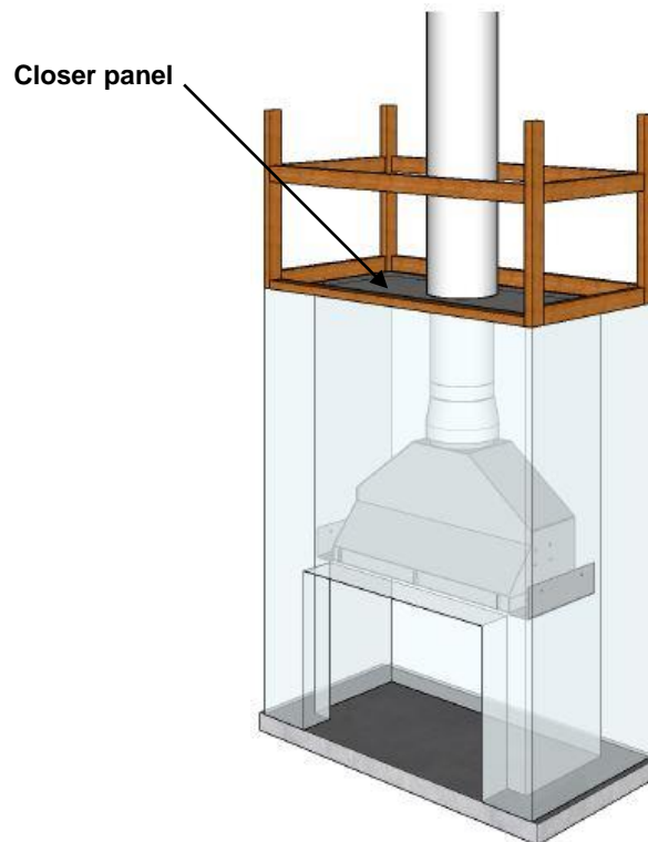
3. Fix the closer panel into position on top of the concrete chimney cavity. Then run the first section of the outer casing onto the closer panel.
