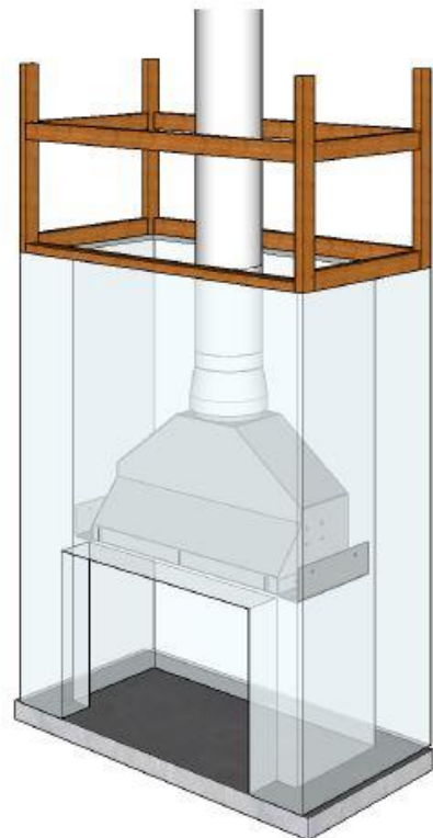
2. Run the first section of inner casing and casing reducer onto gather.
