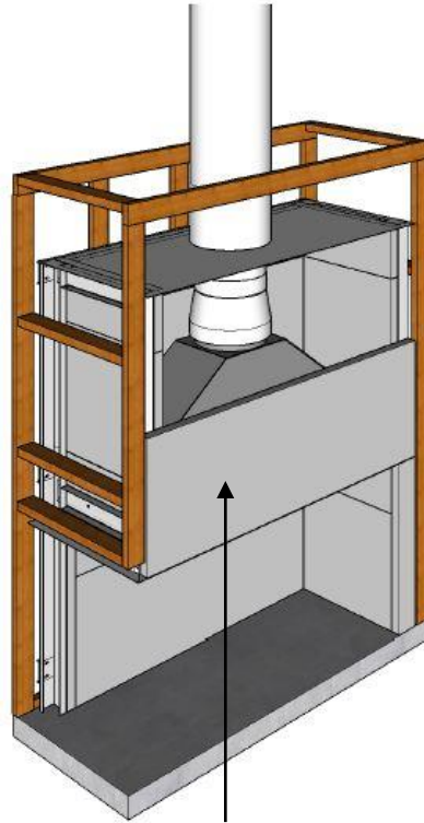
2. Fix front horizontal AAC panels onto steel support frame. 4 x steel screws per panel.
