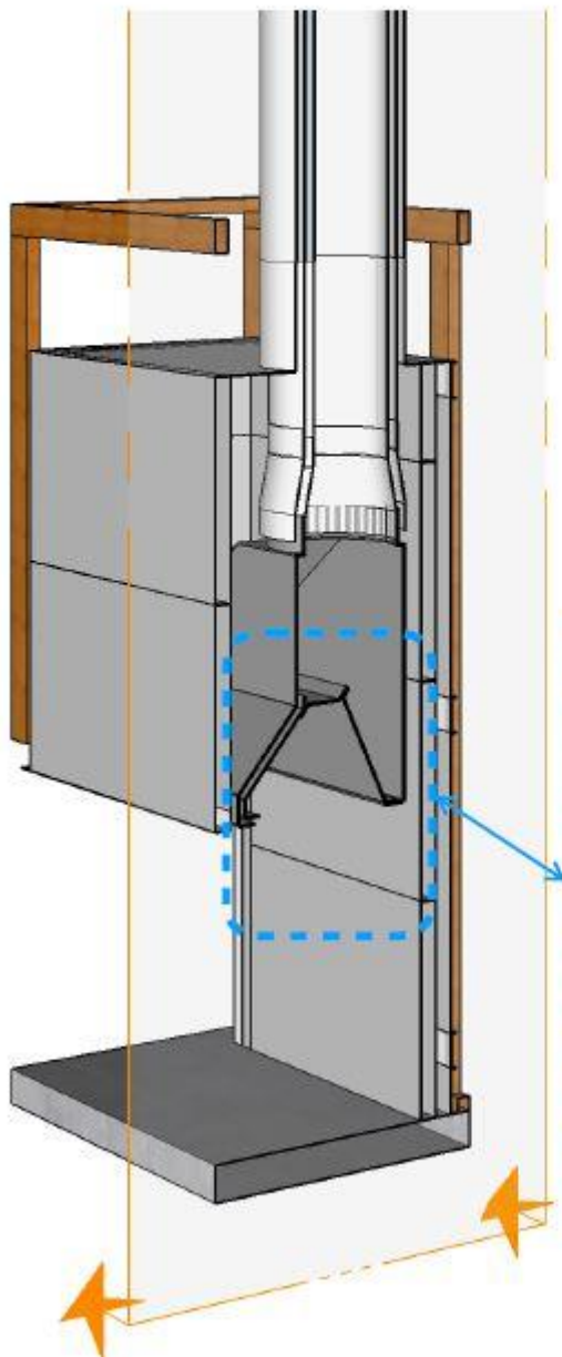
Internal panels in place- cutaway view.
