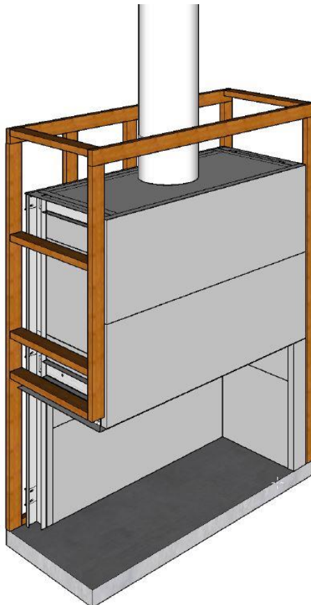
Front AAC panels complete.
