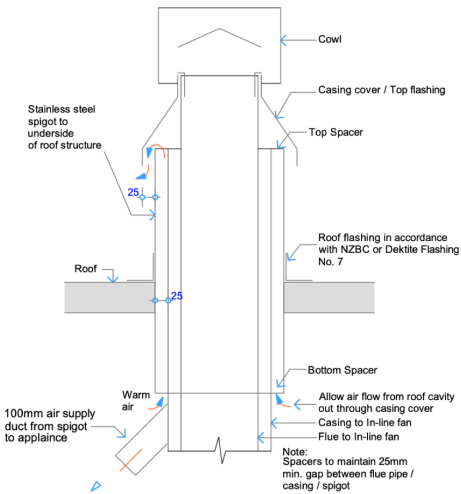
Vertical exit
