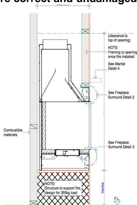
Cross Section - Fire Insert at Floor Level
