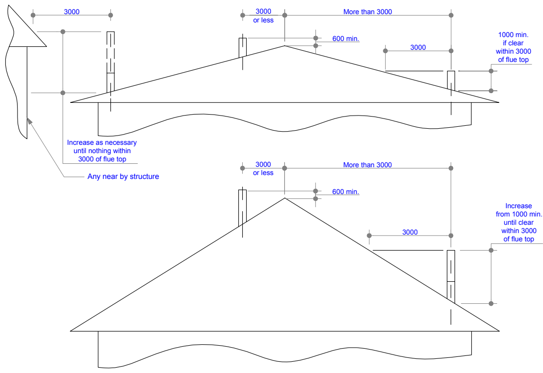
Minimum Height of Flue System Exit Or as per AS/NZS 5601
